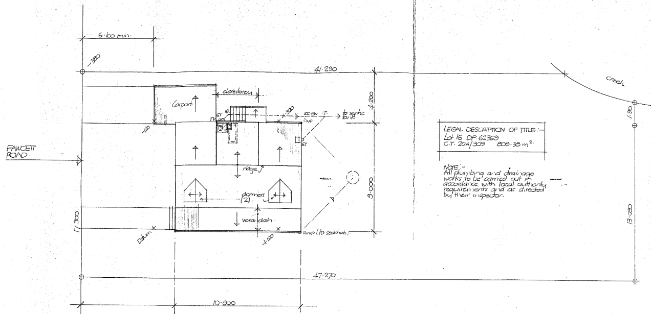
SITE PLAN 1:100.
